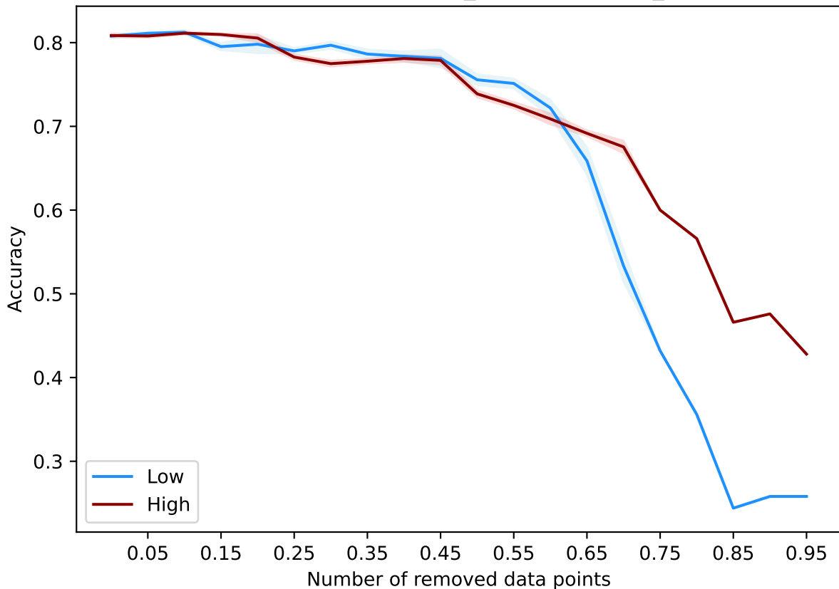
PruningOptimization(optimization_type=size, only_size=100) - pol
